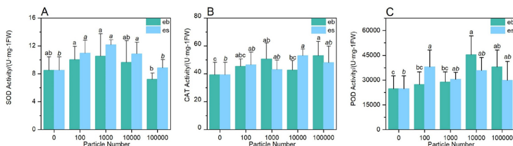
Figure 1. The effects of microbeam radiation on the activities of SOD, POD, and CAT in rice seedling.
